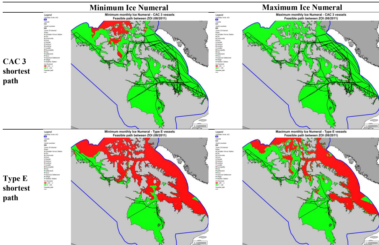
Figure 1. Comparison of monthly aggregated Ice Numerals and feasible shortest path for Type E and CAC 3 ship categories.
