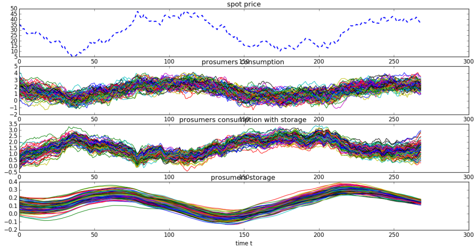
Figure 2: One simulation of spot price (upper graph), prosumers' consumption Q^i (middle graph), prosumer's net consumption Q^i - \alpha^i (lower middle graph) and prosumer's storage level (lower graph) for every prosumers.
