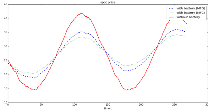
Figure 4: Average spot price over without battery in the system (straight line), with decentralized batteries (dashed line) and with batteries optimized by a central planner (dotted line)
