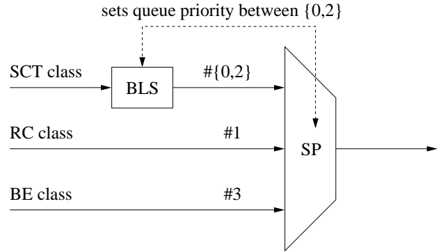
Fig. 2. Burst Limiting Shaper on top of NP-SP at the output port
