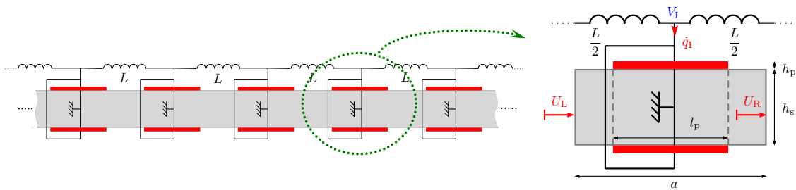
Figure 2: Rod covered with an array of interconnected piezoelectric patches.
