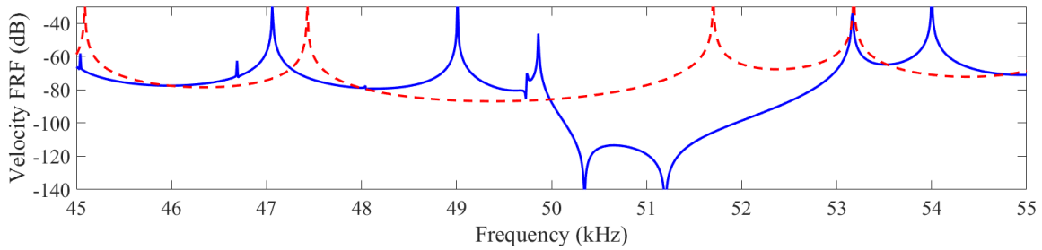
Figure 6: Frequency response function - (---) without network, (—) with L = 1.2 mH.
