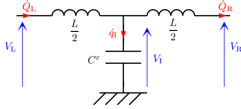
Figure 3: Electrical unit cell without piezoelectric coupling.
