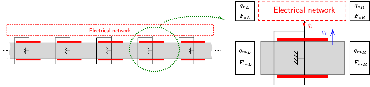
Figure 1: Interconnected array of piezoelectric patches and corresponding electromechanical unit cell highlighting left and right degrees of freedom.
