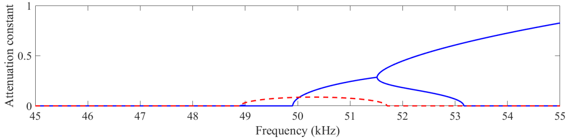
Figure 4: Attenuation constants - (---) without network, (—) with L = 1.2 mH.
