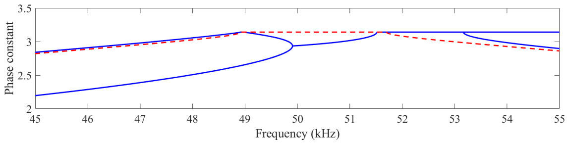
Figure 5: Phase constants - (---) without network, (—) with L = 1.2 mH.
