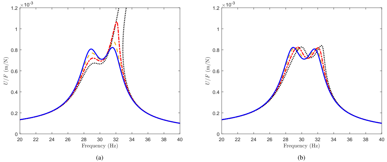
Figure 2: Simulated frequency response functions for various forcing amplitudes, F = 0.2 N ( \text{—} ), F = 0.4 N ( \text{-- --} ), F = 0.6 N ( \text{- . - .} ) and F = 0.8 N ( \cdots ): (a) linear shunt, (b) NPTVA that satisfies Equation (3).
