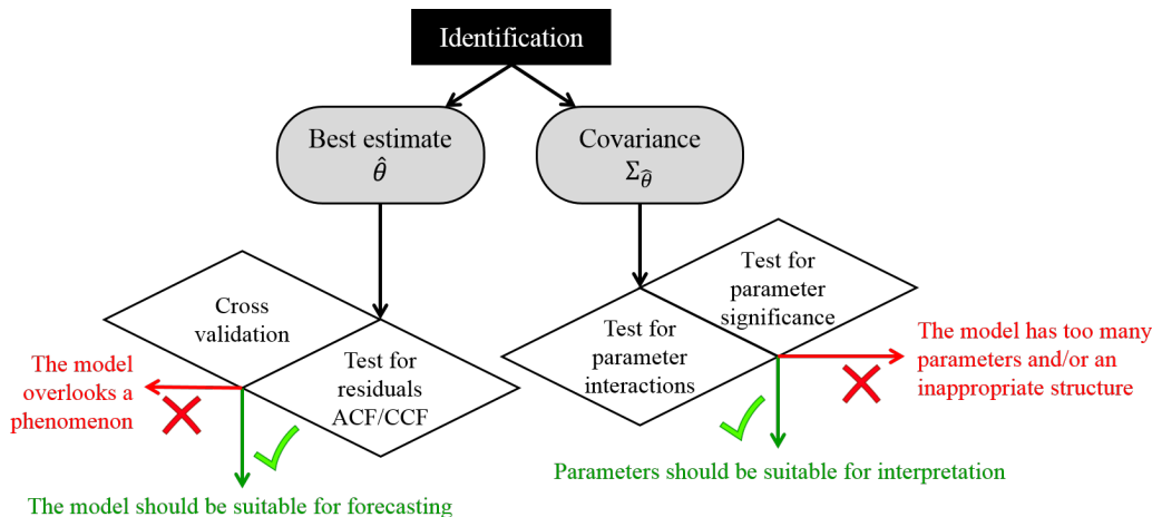
Figure 4: Validation steps
