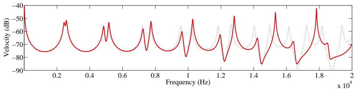
Figure 4: Response functions at low frequencies - ( \cdots ) for the discrete model, ( — ) for the piecewise homogenized model.
