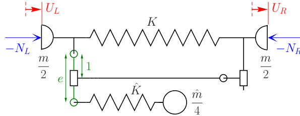
Figure 2: A tuned mass damper fixed to each unit cell
