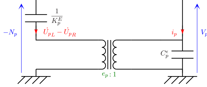
Figure 8: Global model of the piezoelectric element
