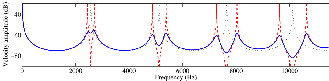
Figure 5: Multimodal damping - ( \cdots ) for e = 0 , ( -\cdot- ) for e = 1, c = 0 and ( — ) for e = 1, c = 1
