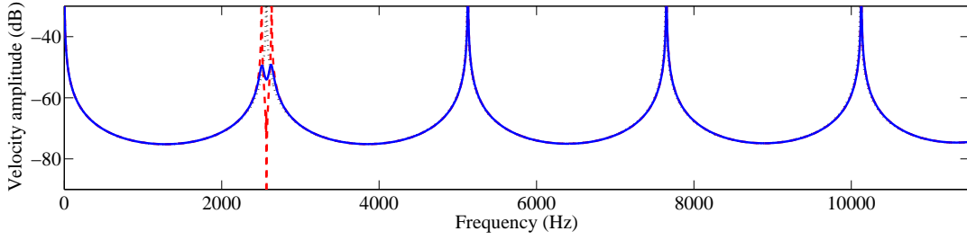
Figure 3: Distributed tuned mass dampers - ( \cdots ) for e = 0 , ( -\cdots ) for e = 1 , c = 0 and ( — ) for e = 1 , c = 1
