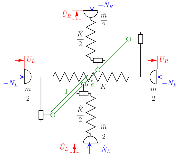
Figure 4: Unit cell for two coupled discretized rods
