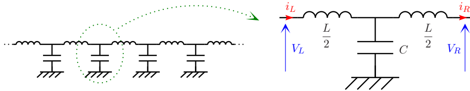
Figure 6: Electrical equivalent of the discretized rod and the corresponding unit cell
