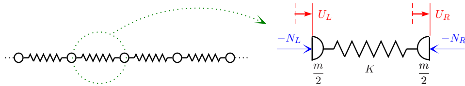
Figure 1: Unit cell of a discretized rod
