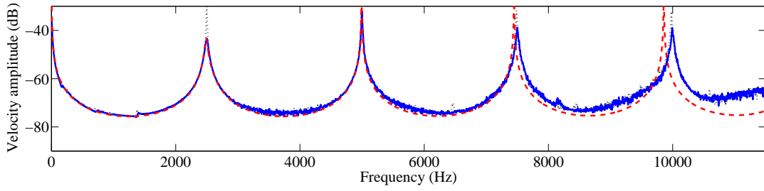
Figure 11: Frequency responses for the distributed shunts strategy - ( \cdots ) for short circuits, ( \text{—} ) for resonant shunts and ( \text{-- --} ) for the discretized model with resonant shunts
