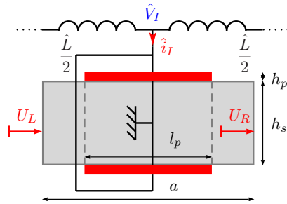
Figure 9: Unit cell of the coupled problem
