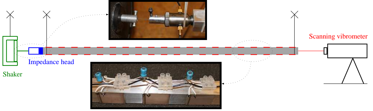
Figure 10: Experimental setup
