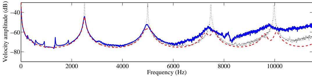
Figure 12: Frequency responses for the multimodal damping strategy - ( \cdots ) for short circuits, ( \text{—} ) for the optimal network and ( \text{-- --} ) for the discretized model with the optimal network
