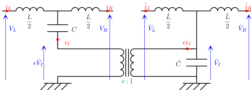
Figure 7: Coupling of two electrical networks
