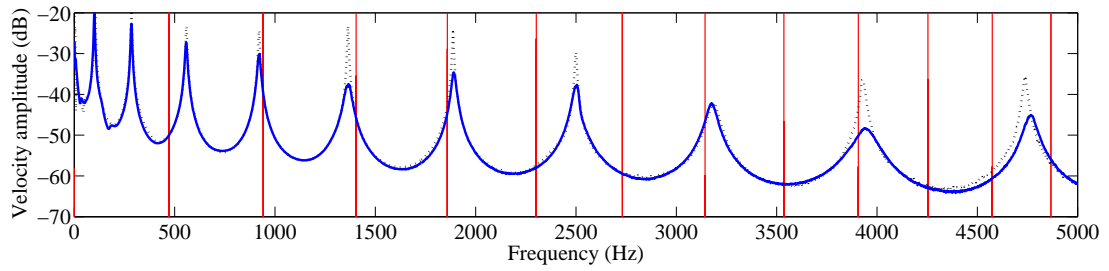
Figure 13: Frequency responses in bending with the non-optimal network - ( \cdots ) for short circuits, ( \text{—} ) for the non-optimal network and ( \text{—} ) for the position of the electric modes
