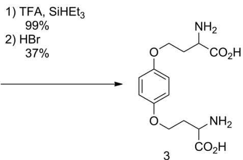
Scheme 5. Synthesis of 3 .
