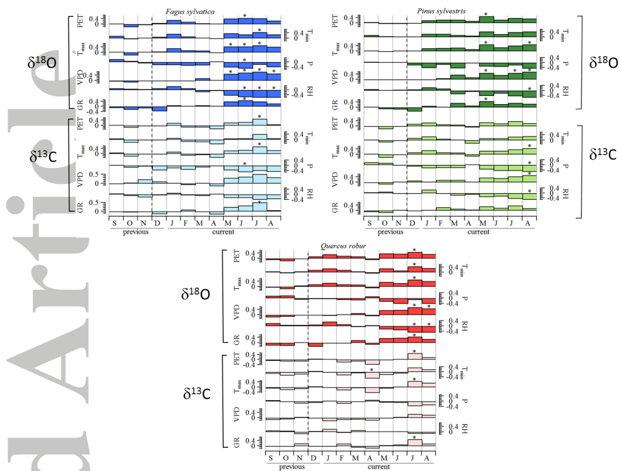
Figure 6: Correlations between species \delta^{18}\text{O} (in ‰; bright colours) and \delta^{13}\text{C} (in ‰; pale colours) chronologies and monthly local climate variables for the 1960-2007 period. Correlations correspond to a 12 months window from September of the previous year to August of the current year. Stars denote correlations significant at 99% confidence interval. GR: Global radiation (in \text{MJ}\cdot\text{m}^{-2}\cdot\text{day}^{-1} ); RH: relative humidity (in %); VPD: vapour pressure deficit (in kPa); P: precipitation (in mm); T_{\max} , T_{\min} : maximum and minimum temperature (in ^{\circ}\text{C} ).
