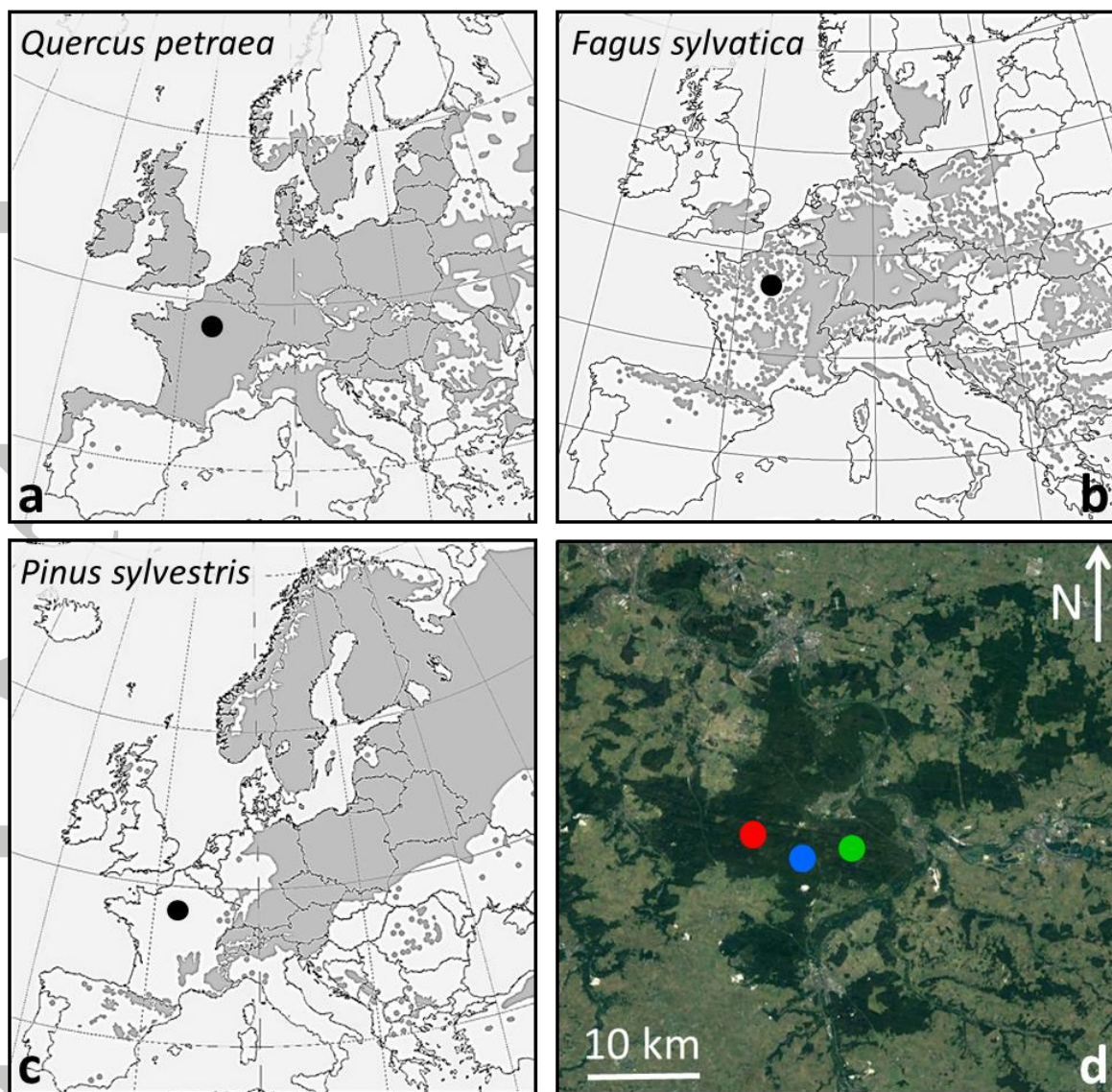
Figure 1: Natural distribution of a) Quercus petraea , b) Fagus sylvatica and c) Pinus sylvestris in Europe (from http://www.euforgen.org/distribution-maps/ ) and location of the study site (black point); d) Sampling sites in Fontainebleau forest (Red: Quercus petraea , blue: Fagus sylvatica and green: Pinus sylvestris ).
