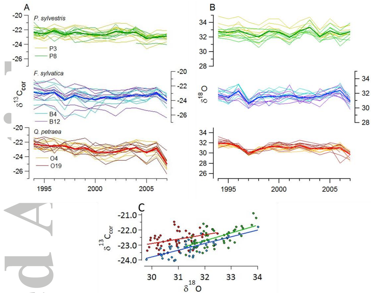
Figure 3: (A) and (B): \delta^{13}C_{cor} and \delta^{18}O chronologies of Q. petraea (cellulose of latewood), F. sylvatica and P. sylvestris (cellulose of total wood) over 1994-2007. Fine lines: individual chronologies (16 trees/species from 2 stands; 1 colour per stand); bold lines: mean chronologies for each species. C: Correlation diagrams of the carbon and oxygen mean isotopic chronologies of Q. petraea (red), F. sylvatica (blue) and P. sylvestris (green). The respective correlation coefficients are R = 0.43, 0.70 and 0.60, p < 0.05 .
