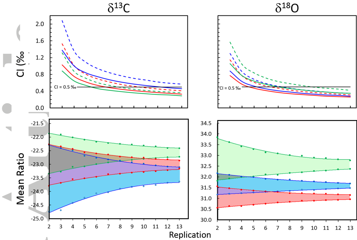
Figure 4: Estimates of the mean values of the CI at confidence levels of 90% and 95% (solid and dotted lines resp., top panel) and ranges of possible mean ratios (bottom panel) for \delta^{13}\text{C}_{\text{cor}} (left column) and \delta^{18}\text{O} (right column) of Q. petraea (red), F. sylvatica (blue) and P. sylvestris (green). The black horizontal lines in the top panels correspond to CI = 0.5‰. The individual chronologies spanning 1994-2007 were used for the calculations.
