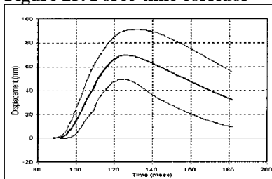
Figure 24. Deflection-time corridor
