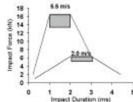
Figure 5. Peak impactor force vs. impact duration.
