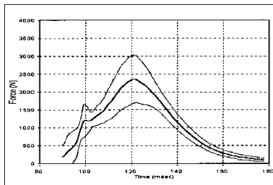
Figure 23. Force-time corridor
