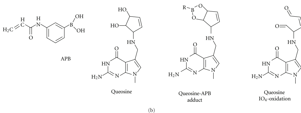
FIGURE 9: Reaction of guanosine residues in RNA with glyoxal and stabilization of the resulting adduct by boric acid \text{H}_3\text{BO}_3 . Inosine residues do not form the stable product under similar conditions (a). Organic derivative of boric acid ( N -acryloylamino)phenyl-3-boronic acid (APB) and its complex with cisdiols present in queosine and the dialdehyde resulting from periodate oxidation of the cisdiol (b).
