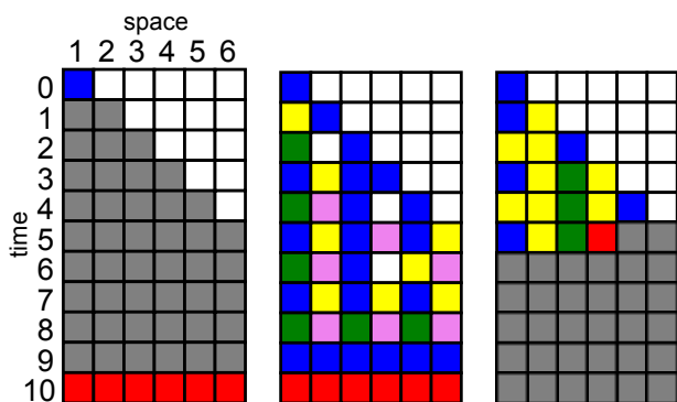
Figure 1: Space-time diagrams of the FSSP for a line of length n = 6 in minimal time 2n - 2 . The quiescent state is white, the initiator state (general state) is blue, and the firing state is red. Grey cells are still undefined. On the left, the space-time diagram is an illustration of the problem with the initial configuration and the expected final state. In the middle, one example of transition function that synchronized correctly in minimal time. On the right an example of rule which failed to synchronize. Indeed, one cell is firing before the other ones.
