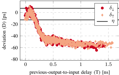
Fig. 9: Fitting an exp-channel involution to measured data.
