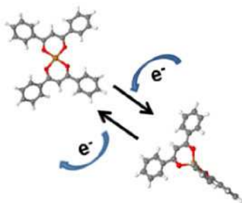
Figure 1. Molecular models of \text{Cu}(\text{dbm})_2 in its neutral and charged configuration.
