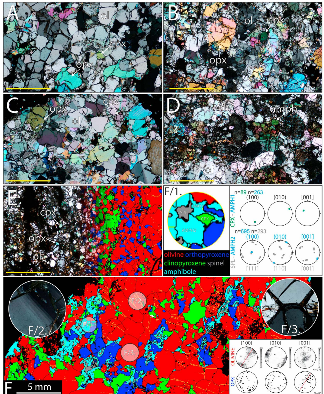
Figure 2. Photomicrographs of representative xenoliths showing coarse-grained protogranular ((a) KPF50420 lherzolite), coarse-grained porphyroclastic ((b) NH1402 lherzolite and (c) NH0601A lherzolite), amphibole-rich ((d) GN1407 amphibole-rich harzburgite), and fine-grained equigranular ((e) GS0611 lherzolite, overlaid by the EBSD phase map) textures. (f) EBSD phase map of porphyroclastic lherzolite TOB1403. Bottom right inset displays the CPOs of olivine and orthopyroxene in this xenolith. Enlargements illustrate typical microstructural features of this sample: F/1: Pole figures indicating topotaxial overgrowth of amphibole onto clinopyroxene and the relationship between spinel and amphibole orientation in an amphibole-bearing spinel-pyroxene cluster. F/2: Subgrain walls in olivine, perpendicular to the foliation plane. F/3: 120° triple junctions between olivine grains indicate annealing.
