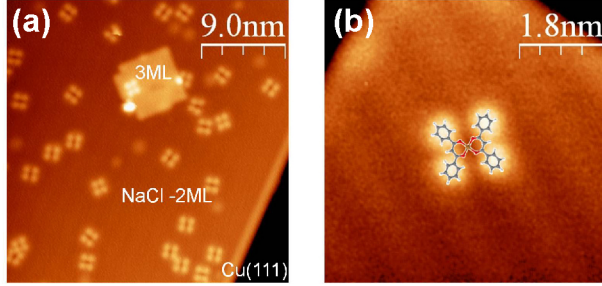
Figure 2: Constant-current STM images of \text{Cu}(\text{dbm})_2 on a bilayer of NaCl on Cu(111) (a) Tunneling current I_t = 1\text{pA} , bias voltage V_t = 1\text{V} . (b) I_t = 700\text{fA} , V_t = 1.2\text{V} .
