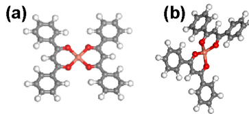
Figure 1: Bis-dibenzoylmethanato-copper C_{30}H_{22}O_4Cu (a) Square-planar complex [Cu(II)(dbm)_2]^0 . (b) Tetrahedral complex [Cu(I)(dbm)_2]^{-1} .
