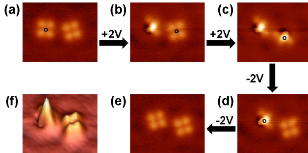
Figure 3: (a)-(e) Sequence of STM images showing the reversible switching of two molecules. The position of the tip above the molecule during the application of the bias voltage is marked by a black circle. (f) 3D representation of image b. Image size: 6.9 nm x 5.5 nm. Imaging conditions: I_t = 400 fA, V_t = 100 mV.
