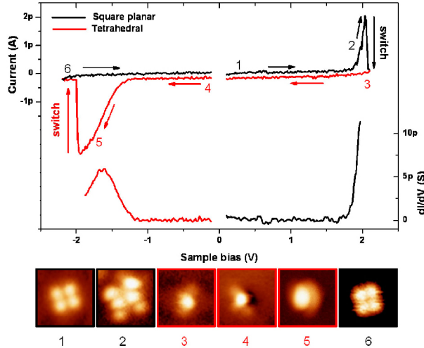
Figure 4: I(V) and dI/dV spectroscopy curves obtained on the SP (black lines) and the Td (red line) molecular species. The numbers that appear on the I-V curves refer to the numbering of the STM images shown below the graph (size: 3.5 nm x 3.5 nm). They are located at the corresponding imaging bias voltage. 1, 2 and 6 (3, 4 and 5) correspond to the SP (Td) species.
