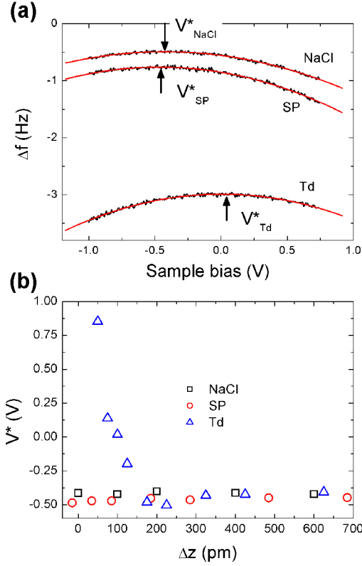
Figure 5: (a) Frequency shift \Delta f as a function of V above NaCl, a SP and a Td molecule. \Delta z = 100 pm. Imaging conditions: oscillation amplitude A = 240 pm, I_t = 700 fA, V_t = 400 mV. Each measurement is fitted with a parabola (red lines). (b) V^*(\Delta z) above NaCl, the SP and the Td molecule.
