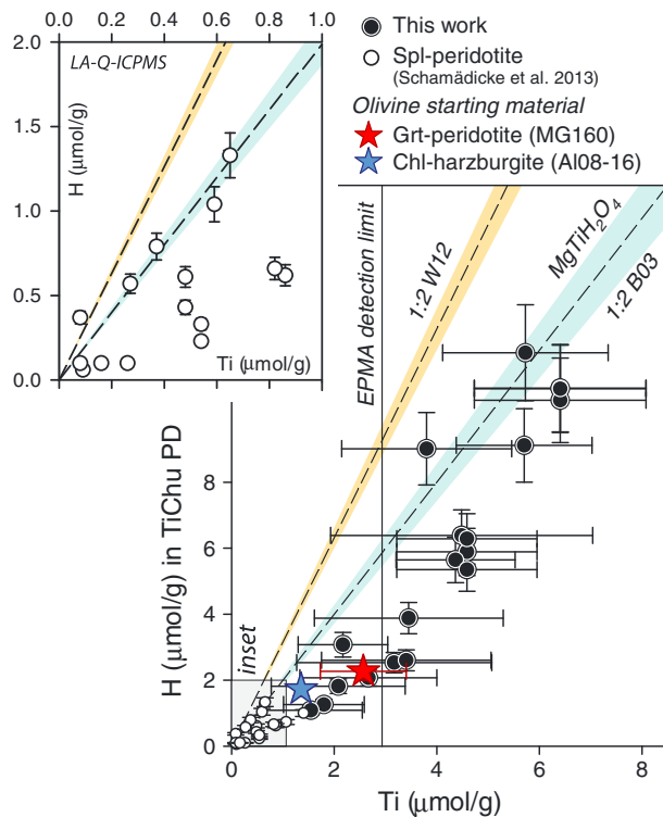
Figure 7. Hydrogen related exclusively to [TiChu-PD] (Bell et al., 2003 calibration) versus titanium in \mu\text{mol/g} from the present experiments (Tables 2 and 3) measured by EPMA, the two starting materials measured by LA-ICPMS (red and blue stars, Scambelluri et al., 2014 and Marchesi et al., 2013, respectively) and data obtained by means of LA-Q-ICPMS for some spinel peridotites (inset, Schmädicke et al., 2013). For comparison the relative position of the 1:2 if the calibration of Withers et al. (2012) is also shown. Note that abundant inclusions of ilmenite rods in MG160 olivine (red star) are observed, therefore contributing to its bulk Ti content.
