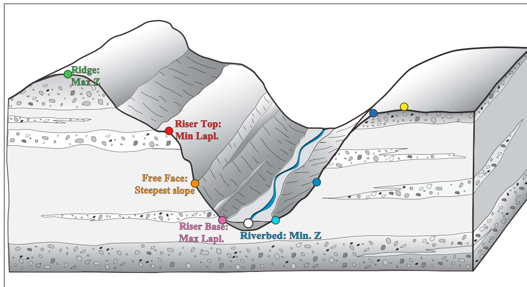
Figure 2. Idealized representation of the nine geometric features identified mathematically by the 3D_Fault_Offsets code.
