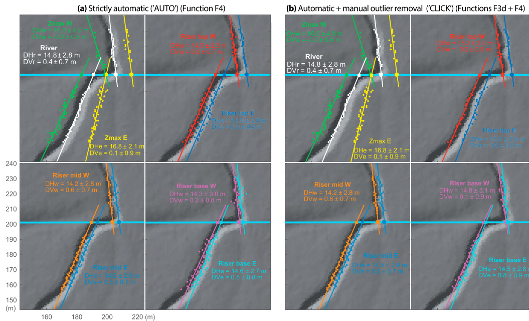
Figure 4. (a) Using the “cleaned” best fit lines, the code calculates the lateral and vertical offsets by subtracting the x and z coordinates of the piercing points of their respective best fit lines on either side of the fault. Uncertainties on the offsets are also calculated. The calculations are here strictly automatic (AUTO approach). (b) Similar offset calculations but performed after the user have manually removed a few outlier points in the point clouds (CLICK approach).
