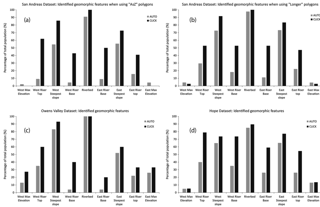
Figure 7. Identified geomorphic features (i.e., with geomorphic relevance) in the three data sets. (a) San Andreas data set (Table ES-A) with measures made using AsZ polygons. (b) San Andreas data set (Table ES-A) with measures made using longer polygons. (c) Owens Valley data set (Table ES-C). (d) Hope data set (Table ES-D). See discussion in text.
