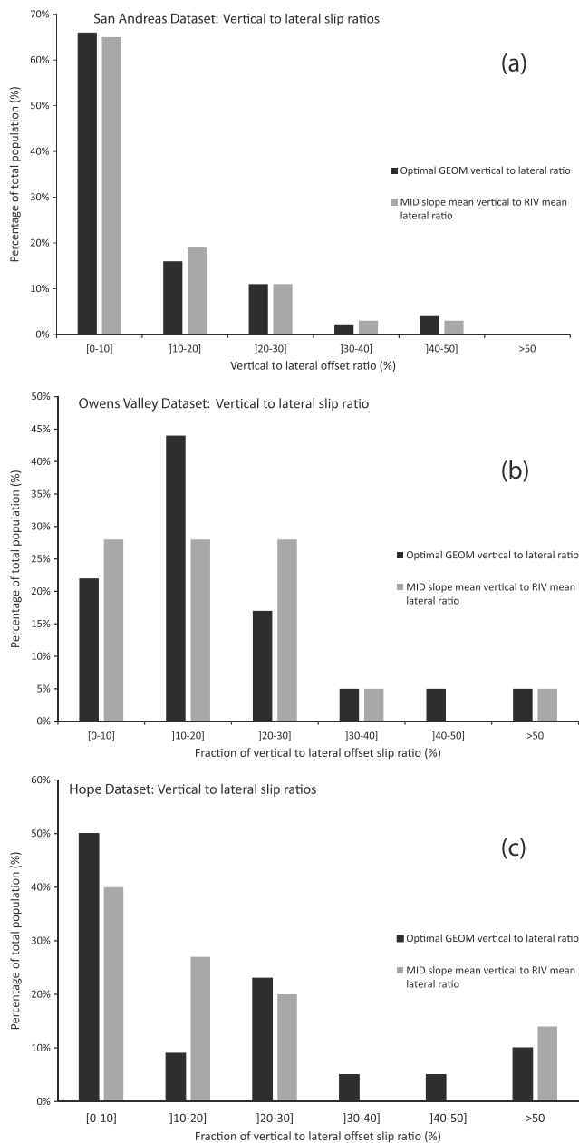
Figure 13. Vertical to lateral slip ratios measured in the three data sets. The ratios are calculated from both the optimal geomorphic offsets (GEOM) and the mean vertical and lateral offsets recorded by the steepest slopes and the riverbeds, respectively.
