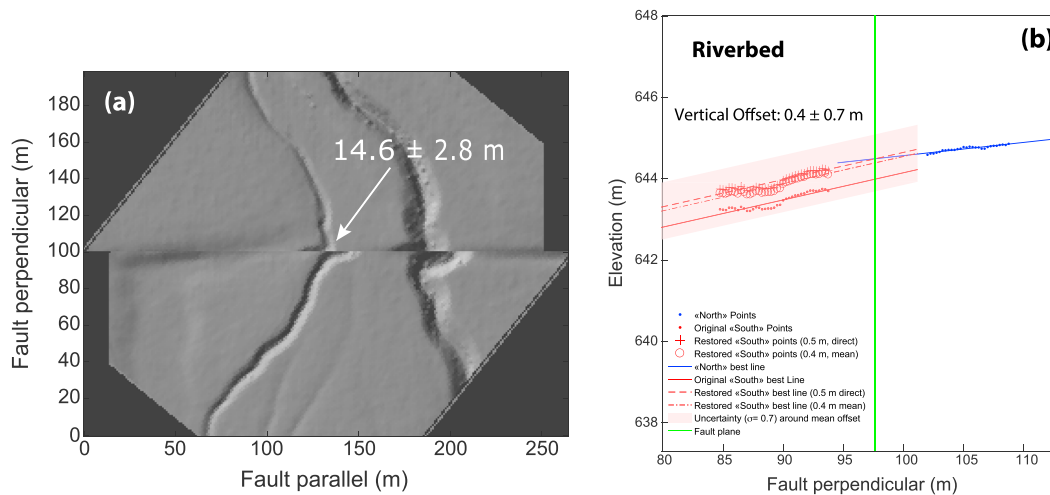
Figure 6. (a) Horizontal back slip of the marker performed by the code, using the offset value provided by the user (here, optimal lateral offset). (b) Vertical back slip of the riverbed of the marker. The back slip is performed using the “direct” vertical offset (see details in supporting information ES1), but the mean vertical offset is shown along with its uncertainty. Here the vertical offset is about null, what explains the large relative uncertainties. Data are in Table ES-B.
