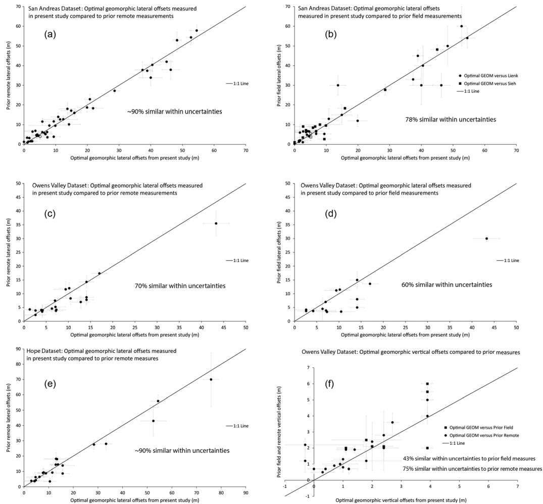
Figure 10. Comparison of geomorphic optimal (GEOM) lateral and vertical offsets obtained in present study with prior field and remote measures. (a) San Andreas data set, lateral offsets compared to prior remote measures. (b) San Andreas data set, lateral offsets compared to prior field measures. (c) Owens Valley data set, lateral offsets compared to prior remote measures. (d) Owens Valley data set, lateral offsets compared to prior field measures. (e) Hope data set, lateral offsets compared to prior remote measures. (f) Owens Valley data set, vertical offsets compared to prior remote measures. The empty symbols indicate poorly constrained lateral offsets with uncertainties \geq 10 m.
