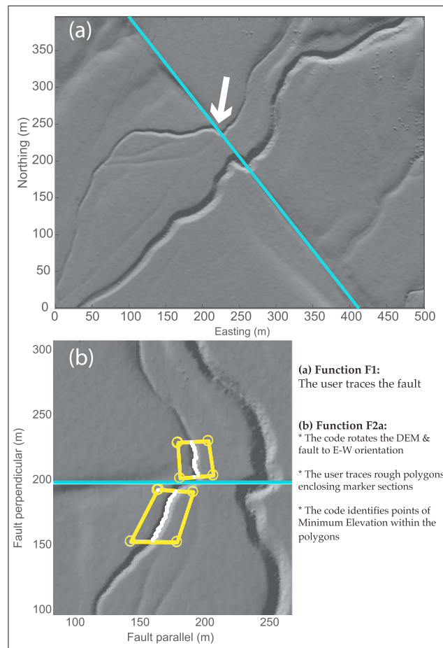
Figure 3. (a) Hillshade representation of a DEM region (here at 1 m resolution) including two offset channels (southern San Andreas Lidar data; Zielke et al., 2012) and fault trace (blue) drawn by the user. The white arrow indicates the ZA6808a marker that is illustrated in following figures. (b) Once the user has traced the fault, the code rotates the DEM and fault to an E-W attitude. When the user has traced the two polygons around the marker sections of interest, the code identifies the points of minimum elevation within the polygons and populates the DEM with those points (white). They underline the riverbed. In this figure and following (Figures 3–6 and additional ones in supporting information ES1), the example has been processed using 1 m resolution Lidar data to enhance the clarity of the figures.
