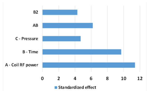
Figure 6. Standardized Pareto chart relative to the memory gate CD
