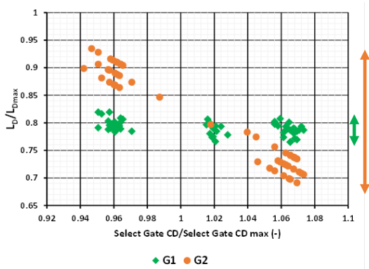
Figure 7. L_D parameter variation before and after using R2R controller
