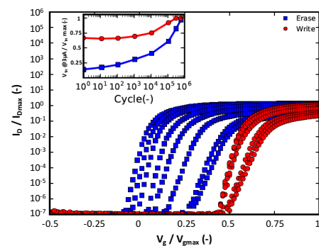
Figure 2. I_D(V_G) distribution during cycling test
