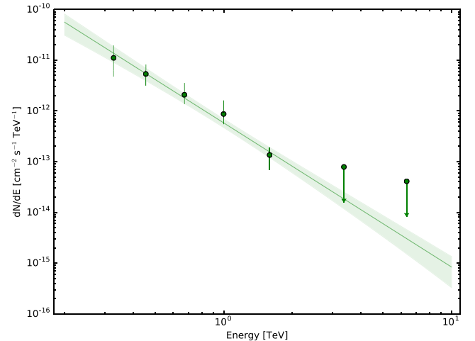
Figure 2. H.E.S.S. spectrum of PKS 0625–354 above 200 GeV. The panel presents best power-law fit to the data as a function of the true energy. Upper limits are given at 99 per cent confidential level with Feldman & Cousins (1998) confidence intervals. The green bow tie area gives the uncertainty of the fit at the 1\sigma confidence level.
