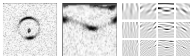
Fig. 2. Example of our feature extraction procedure used to transform a ring. The image on the right shows the response of a set of Gabor filters after convolution with a polar transformed image of an Einstein ring. The strongest response is seen in the orientation perpendicular to the radial direction and at the frequency most closely matching that of the ring.
