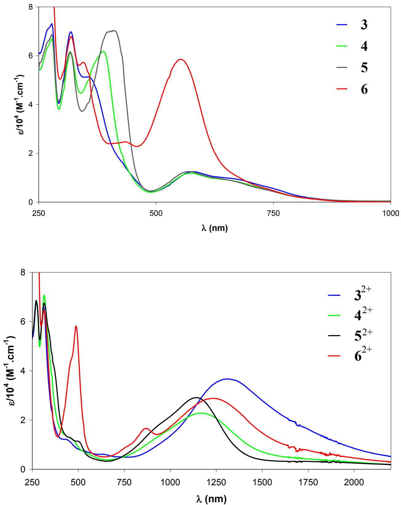
Figure 2 : - (top) UV-Vis-near IR spectra of 3 , 4 , 5 and 6 in DCM. - (bottom) UV-Vis-near IR spectra of 3^{2+} , 4^{2+} , 5^{2+} and 6^{2+} in DCM.
