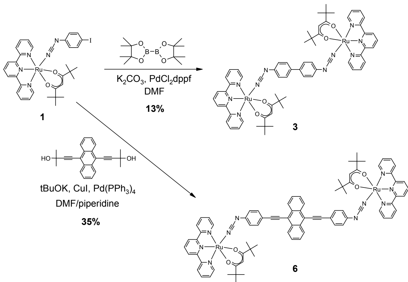
Scheme 2: Synthesis of [ \{\text{Ru}(\text{tpy})(\text{thd})\}_2(\mu\text{-dcbp}) ] 3 and [ \{\text{Ru}(\text{tpy})(\text{thd})\}_2(\mu\text{-bcpea}) ] 6
