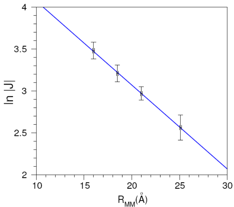
Figure 7 : Decay law of the magnetic coupling versus the metal-metal distance R_{\text{MM}} .
