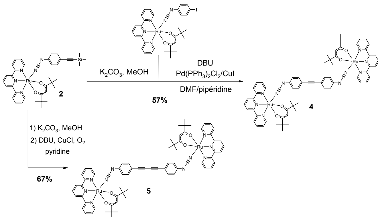
Scheme 3: Synthesis of [ \{\text{Ru}(\text{tpy})(\text{thd})\}_2(\mu\text{-bcpa}) ] 4 and [ \{\text{Ru}(\text{tpy})(\text{thd})\}_2(\mu\text{-bcpda}) ] 5
