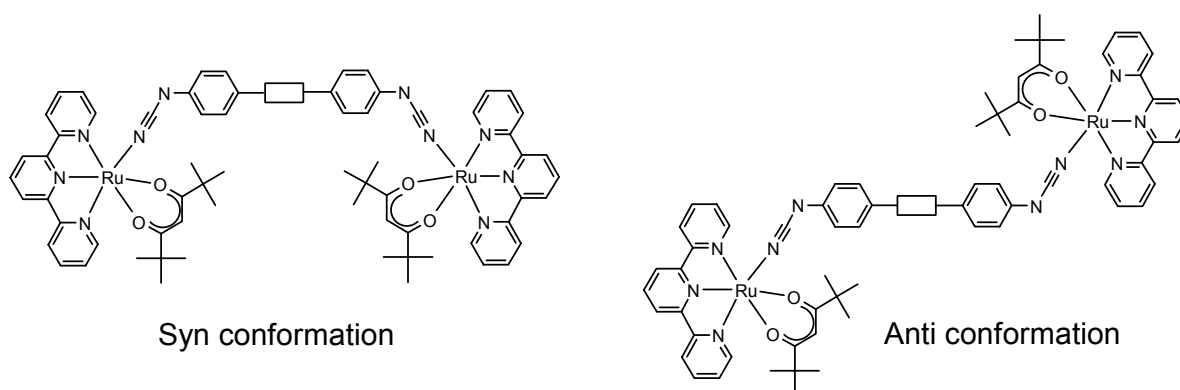
Scheme 4: Syn and Anti conformations of dinuclear compounds.
