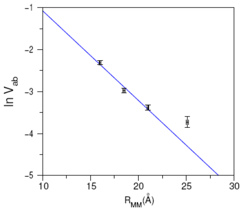
Figure 4 : Decay law for the electronic coupling parameter V_{ab} in log scale vs the metal-metal distance R_{MM} .
