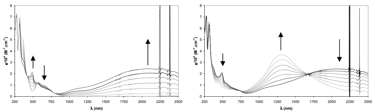
Figure 3 : Spectroelectrochemical oxidation of 3 in DCM, 0.1 M TBAH (electrolysis at 0.46 V vs. SCE). left : \mathbf{3} \rightarrow \mathbf{3}^+ . right : \mathbf{3}^+ \rightarrow \mathbf{3}^{2+} .
