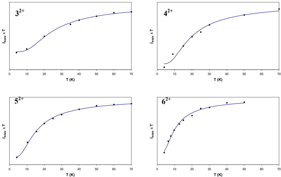
Figure 6 : Double integrated EPR signal intensity times Temperature ( I_{\text{totale}} \times T ) of 3^{2+} , 4^{2+} , 5^{2+} and 6^{2+} versus temperature : experimental (dots) simulated (lines).
