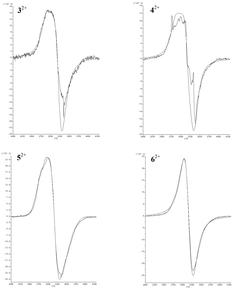
Figure 5 : experimental and simulated EPR spectrum of 3^{2+} , 4^{2+} , 5^{2+} et 6^{2+} in frozen DCM solution (30 K).
