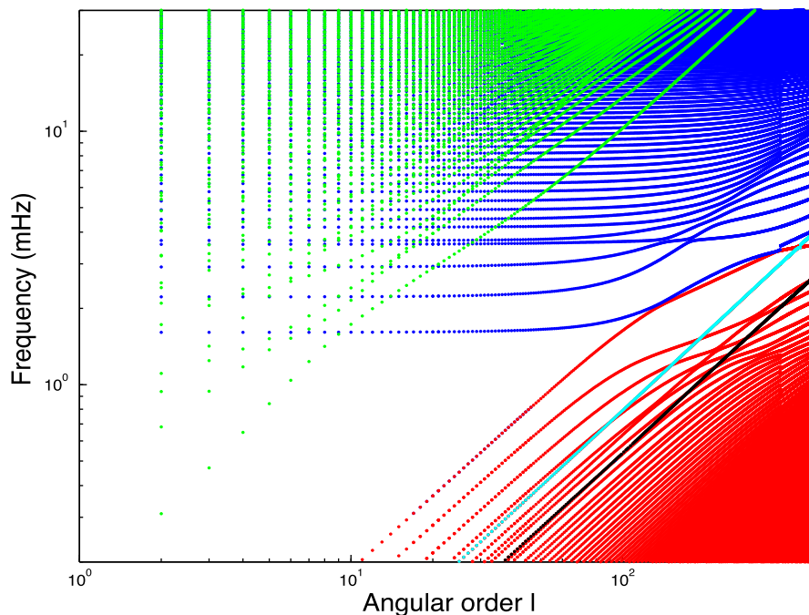
Figure 1. Dispersion of normal modes of the full Earth system for the 0.1–30 mHz frequency range. Atmospheric gravity modes (G) are plotted in red, Rayleigh modes (R) in green, atmospheric acoustic (A) modes in dark blue, Lamb modes (L) in light blue and tsunami modes (T) in black.
