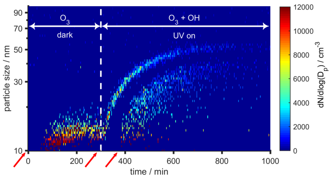
Fig. 4 Number particle size distribution after ozone injection as a function of time for a chamber experiment. Red arrows indicate ozone injections (reaching ca. 600 ppb v ). Biofilms were irradiated prior to ozone injection for 67 hours to induce VOC production. After 300 min of dark ozonolysis, the UV lights were turned on together with a second ozone injection to initiate OH radical chemistry. At minute 380, ozone was injected a third time.
