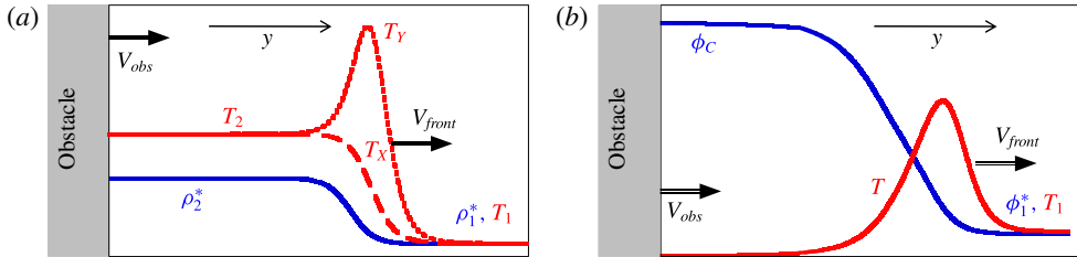
FIGURE 1. (Colour online) Schematic of density and temperature profiles generated by a moving obstacle in the y -direction in a one-dimensional medium. (a) Molecular gas: T_Y and T_X are the longitudinal and transverse temperatures. The gas density \rho is the blue curve. (\rho_1^*, T_1) and (\rho_2^*, T_2) are respectively the density and temperature values of supersonic and subsonic gases on either side of the shock front linked by Rankine–Hugoniot conditions (see § 2). (b) Granular gas: T is the temperature. The gas volume fraction \phi is the blue curve. (\phi_1^*, T_1) are the initial value of volume fraction and temperature. \phi_C is the random close-packing volume fraction.
