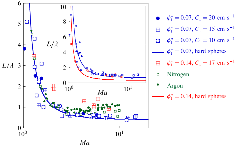
FIGURE 9. (Colour online) Shock width normalized by the mean free path \lambda = d/6\sqrt{2}\phi_1^* versus Ma for \phi_1^* = 0.07 and C_1 = 0.1, 0.15, 0.2 \text{ m s}^{-1} (blue symbols) and \phi_1^* = 0.14 and C_1 = 0.175 \text{ m s}^{-1} (red symbols). The blue line gives the resolution of the Mott-Smith model for a gas of hard spheres. To compare to molecular gases, green symbols give the shock widths measured in argon and nitrogen (Alsmeyer 1976). Inset: the shock width normalized by the bead diameter d versus Ma . The lines give the resolution of the Mott-Smith model for a gas of hard spheres. It should be noted that for large Mach numbers and for both volume fraction shock width becomes approximately half the size of the bead.
