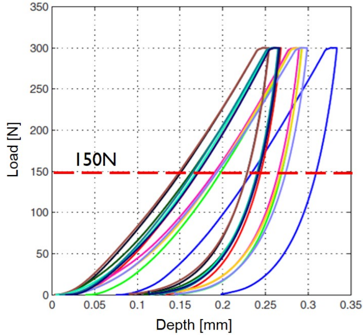
Figure 1: Indentation test on friction material on different locations
