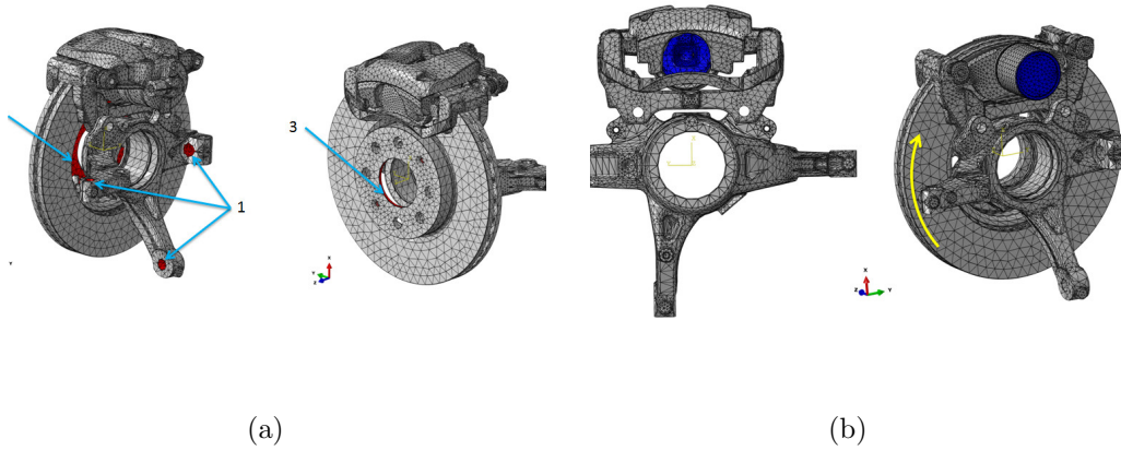
Figure 11: Boundary conditions on the brake system model: (a) Boundary Conditions, (b) Loading
