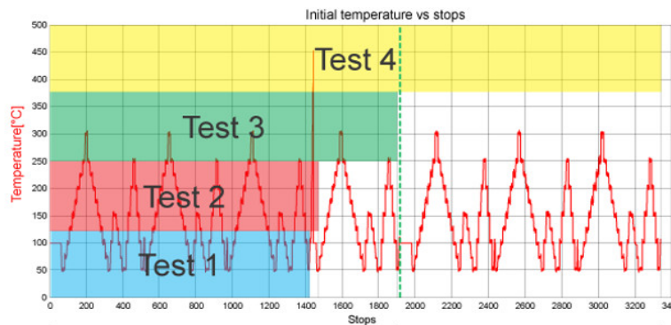
Figure 5: Test procedure description
