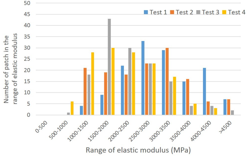
Figure 7: Cluster of elastic modulus per sliding state
