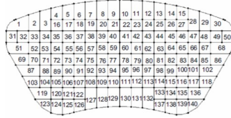
Figure 3: Mapping of the friction pad for indentation tests
