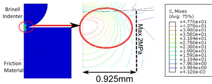
Figure 1: Indentation test on friction material on different locations
