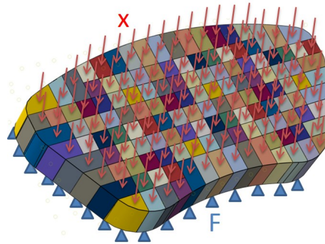
Figure 7: Cluster of elastic modulus per sliding state
