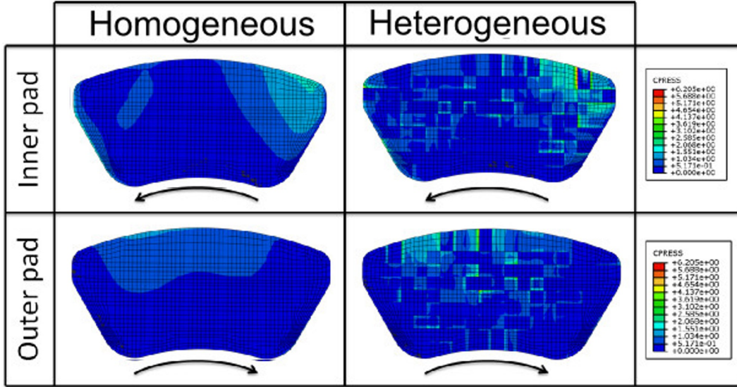
Figure 12: Pressure distribution of homogeneous and heterogeneous cases for the configuration 1
