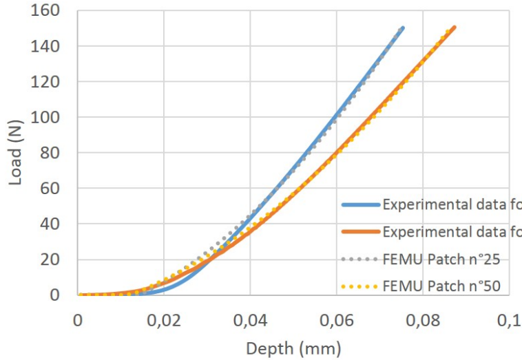
Figure 4: Inverse identification with FEMU method on patch n^{\circ}25 and n^{\circ}50
