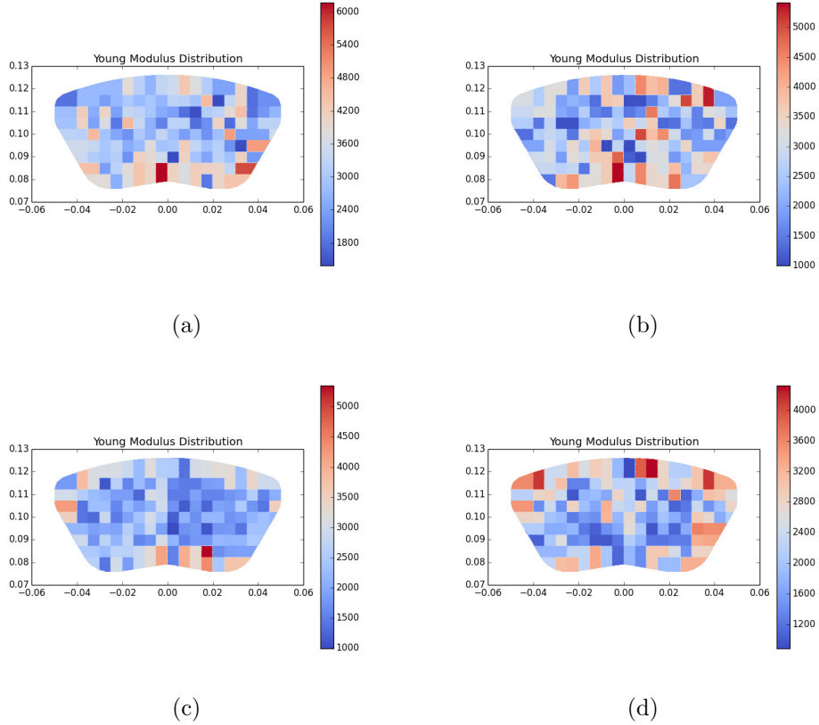
Figure 6: Young Modulus (MPa) Distribution after different tests: (a) Test 1, (b) Test 2, (c) Test 3, (d) Test 4
