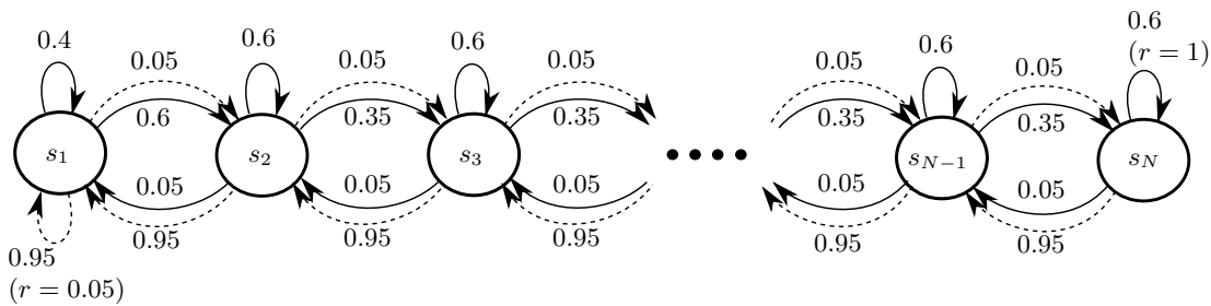
Figure 1: The N -state Ergodic RiverSwim MDP
