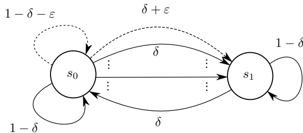
Figure 2: The MDP M' for lower bound (Jaksch et al., 2010)
