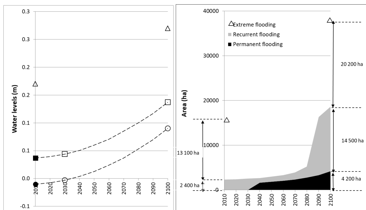
Fig. 2 Evolution of (a) water levels and (b) coastal flooding area resulting from PF, RF and EF over time.
