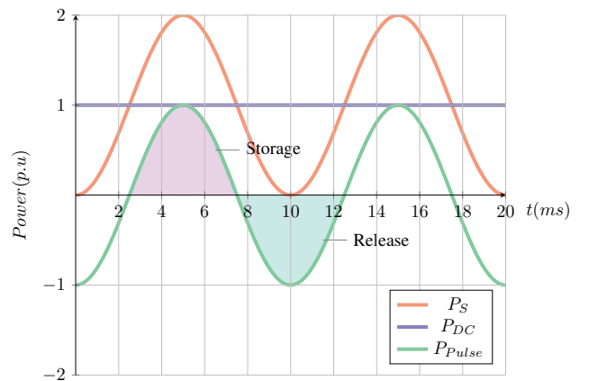
Fig. 1: Typical power waveforms for an AC/DC converter. P_S is the power on the AC side, P_{DC} is the power on the DC side and P_{Pulse} is the power that needs to be buffered by the PPB.
