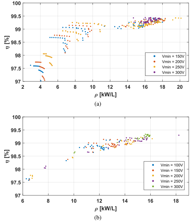
Fig. 8: Results of the optimisation presented in the Power Density vs. Efficiency domain. a) X6S capacitor/planar inductor with a thermal coefficient of 5 cm 3 /W for the cooling system. b) X6S capacitor/PCB-embedded inductor with thermal coefficient of 5 cm 3 /W.
