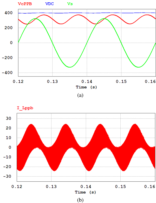
Fig. 9: PSIM simulation of the optimised PPB. a) Voltage waveforms. b) Inductor current waveforms. Note that the current changes its sign during each switching period allowing ZVS.
