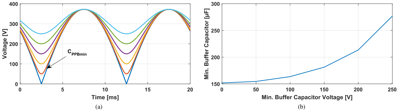
Fig. 5: Impacts of minimal voltage value a) Waveforms. b) Buffer capacitor value
