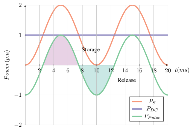
Fig. 1: Typical power waveforms for an AC/DC converter. P_S is the power on the AC side, P_{DC} is the power on the DC side and P_{Pulse} is the power that needs to be buffered by the PPB.
