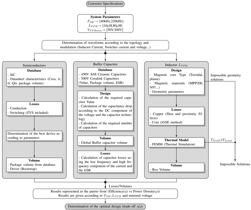
Fig. 4: Design Flow Chart presenting the optimization procedure implemented for the Buck PPB
