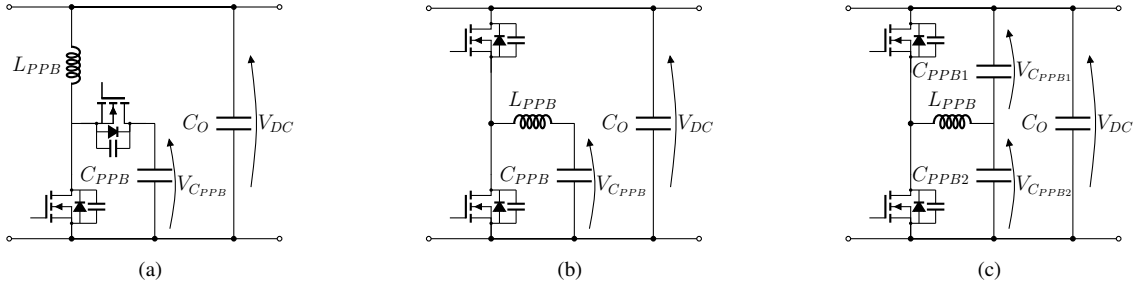
Fig. 2: Examples of different parallel Power Pulsating Buffers. a) Boost b) Buck c) Symmetrical Half Bridge (HB)
