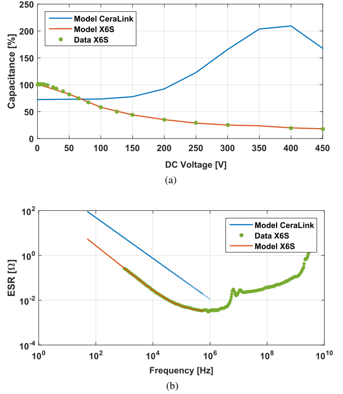
Fig. 7: X6S and CeraLink models implemented in the design procedure, data for X6S are available thus a comparison with the model is possible a) Capacitance models. b) ESR models.
