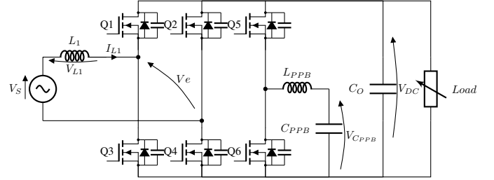
Fig. 3: A full-bridge PFC stage with the considered PPB for output decoupling
