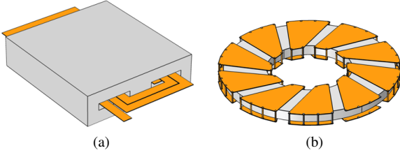
Fig. 6: PCB inductor technologies. a) Planar PCB inductor. b) PCB-embedded inductor.
