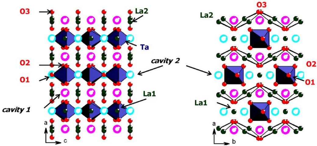
Fig. 1. \text{La}_3\text{TaO}_7 crystalline structure in \text{Cmcm} space group with evidence of two cavities.
