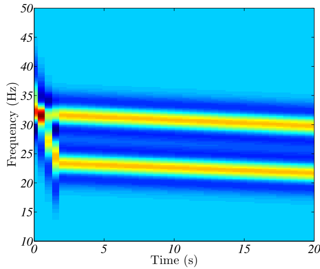
FIGURE 13— Time-frequency kernel used for the detection of “Madagascar” pygmy blue whale calls (unit B) with Mellinger and Clark’s method [9].
