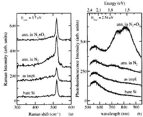
FIG. 3. (a) Raman and (b) PL spectra of Si implanted \text{SiO}_2 layers for different annealing conditions.
