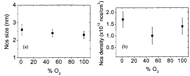
FIG. 7. Evolution of (a) the NC mean radius and (b) NC density vs the O 2 content, as measured on plan-view PEELS-STEM images. The samples have been implanted at 1 keV with a dose of 2 \times 10^6 cm -2 , annealed under N 2 during 30 min at 1050 °C and under N 2 -diluted O 2 with 1.5% O 2 , 50% O 2 , and 100% O 2 at 900 °C for 30 min.
