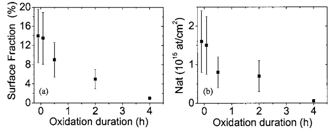
FIG. 3. Evolution of (a) the percentage of surface occupied by Si NCs (coverage) and (b) of the number of silicon atoms within the NCs vs the annealing time under N_2+O_2 , deduced from the images in Fig. 1.
