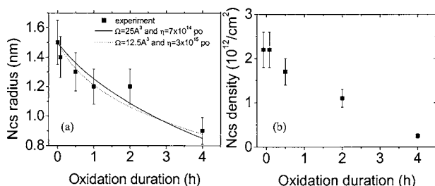
FIG. 2. Evolution of (a) the Si NC mean radius and (b) of the NC aerial density vs annealing time under N_2+O_2 , as measured on the images in Fig. 1. In (a) the model predictions for \Omega=25 \text{ \AA}^3 and \Omega=12.5 \text{ \AA}^3 are plotted in the solid and dashed lines, respectively.
