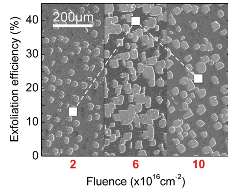
FIG. 4. (Color online) SEM micrographs of the samples annealed at 700 \text{ }^\circ\text{C} during 1800 s. The exfoliation efficiency values are plotted as a function of the total fluence superimposed to the respective sample image.
