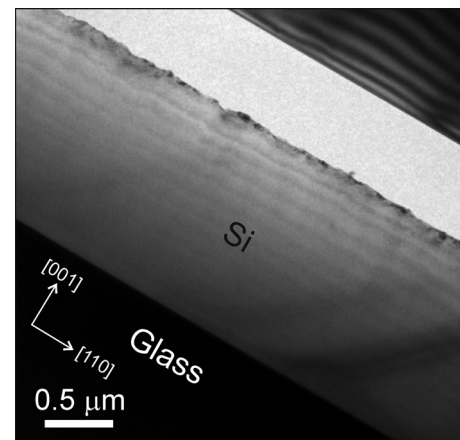
FIG. 5. Cross sectional TEM micrograph of a \approx 1.5 \text{ } \mu\text{m} thick Si film transferred onto a glass substrate.
