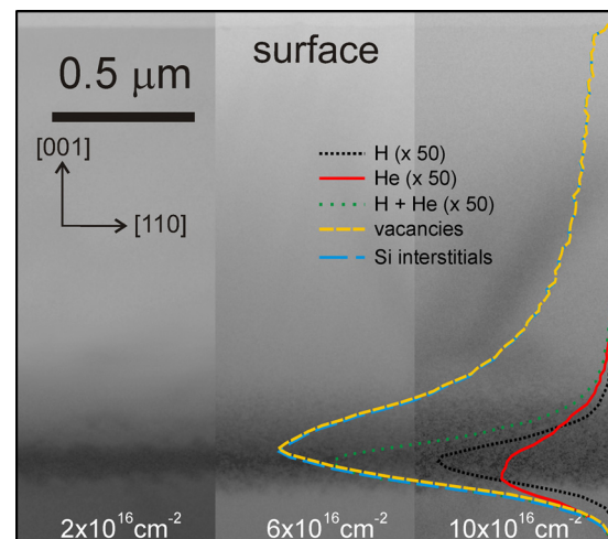
FIG. 2. (Color online) Low magnification cross sectional TEM micrographs of the samples implanted to \Phi = 2, 6, and 10 \times 10^{16} cm -2 and annealed at 350 °C for 1800 s. The superimposed curves are the calculated profiles of the implanted ions and lattice damage.
