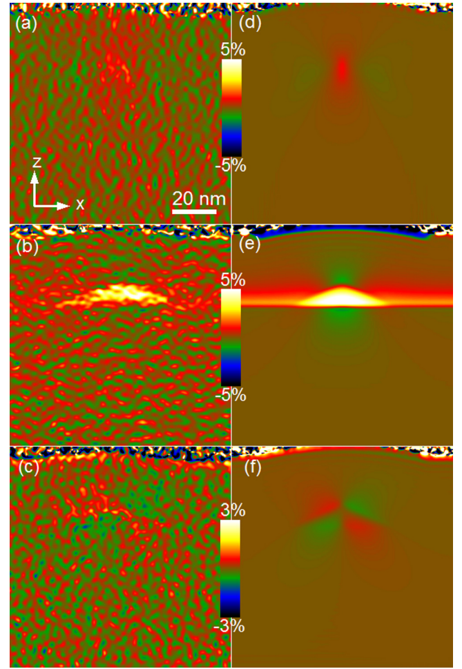
FIG. 4. (a) \varepsilon_{xx}^{rel} , (b) \varepsilon_{zz}^{rel} , and (c) \varepsilon_{xz}^{rel} components of the QD strain field mapped by dark-field electron holography. The corresponding calculated maps are shown in (d) for \varepsilon_{xx}^{rel} , (e) for \varepsilon_{zz}^{rel} , and (f) for \varepsilon_{xz}^{rel} .
