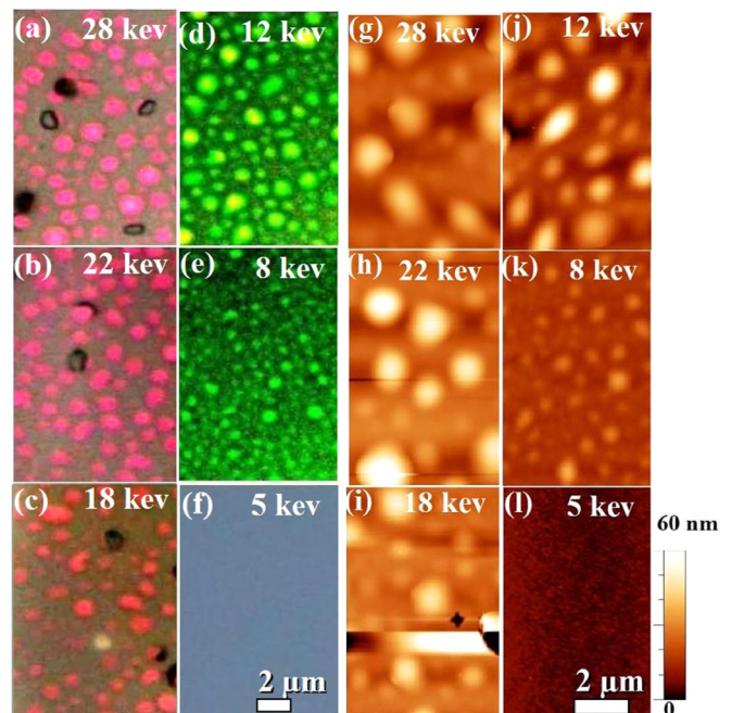
FIG. 1. Optical [(a)–(f)] and AFM [(g)–(l)] images of the samples sequentially implanted He-first with E He indicated in the images and annealed at 550 °C for 30 min.
