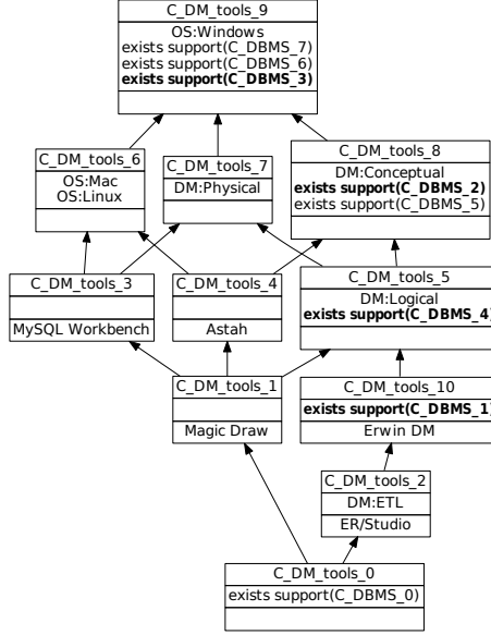
Fig. 2. Concept lattice of the extended context DM\_tools^+
