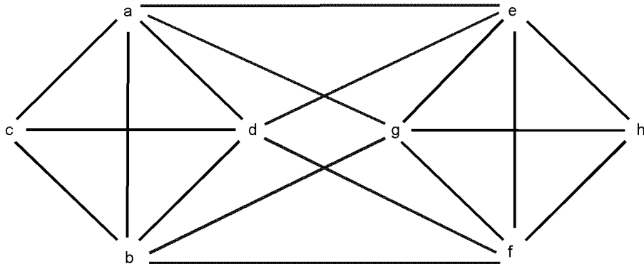
Figure 3: A 1-planar drawing of a planar graph H .
