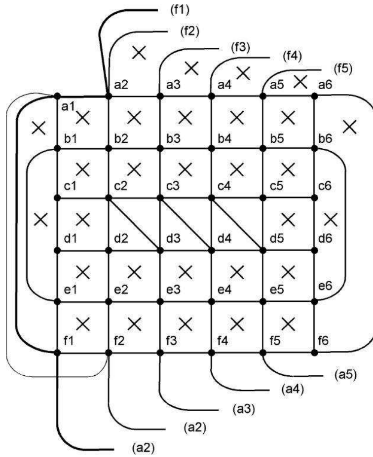
Figure 1: The graph G_6 .
