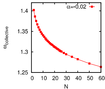
FIG. 20. The collective frequency is plotted as a function of total number of rowers N . The rowers are placed on a regular lattice with lattice constant d = 1 . The data are averaged over 1000 initial configurations. It decays with system size N .
