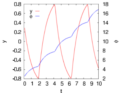
FIG. 2. The periodic beating of a single rowler is plotted as function of time t . The red curve is the displacement y of the rowler, and the blue curve is its phase representation according to Eq. (6).
