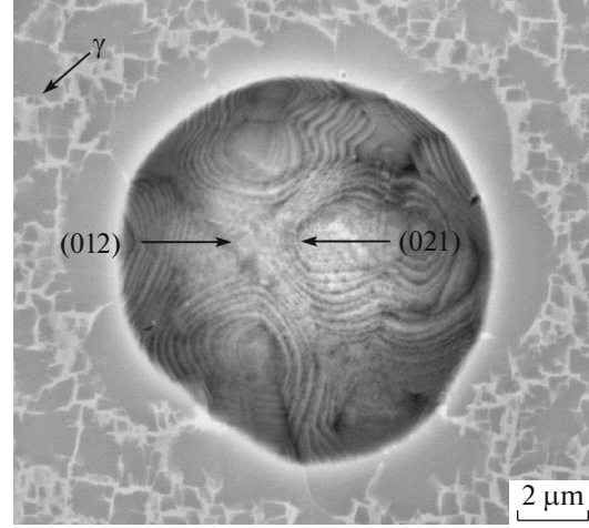
Fig. 5. Pore faceted with \{012\} planes in the single crystal of CMSX-4 alloy after 0.5 h of HIP at 1288^\circ\text{C}/103 \text{ MPa} . There is a \gamma shell around the pore. Section (012), SEM, BSE.
