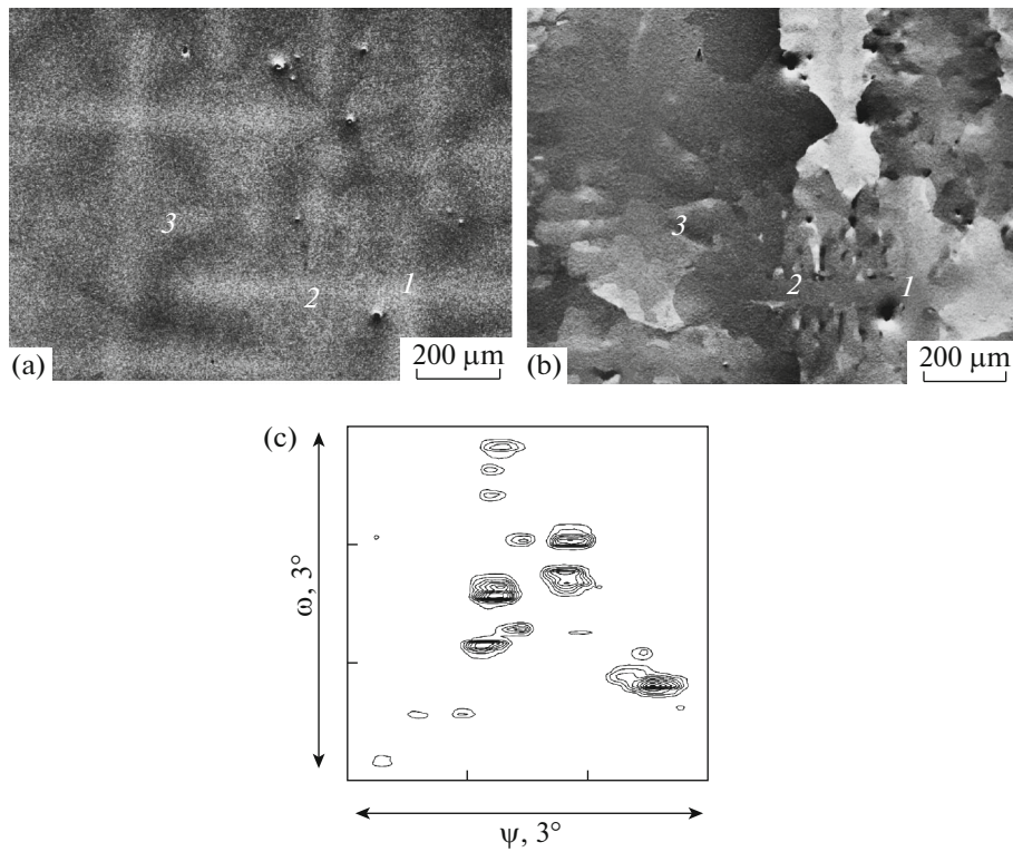
Fig. 3. The subgrain structure of the single crystal of CMSX-4 alloy at cross section (001): (a) BSE contrast by mean atomic number, (b) orientation contrast FSE (numerals 1, 2, and 3 correspond to dendritic arm of first, second, and third orders, respectively), and (c) X-ray orientation scan with area about 1 \text{ mm}^2 [21].
