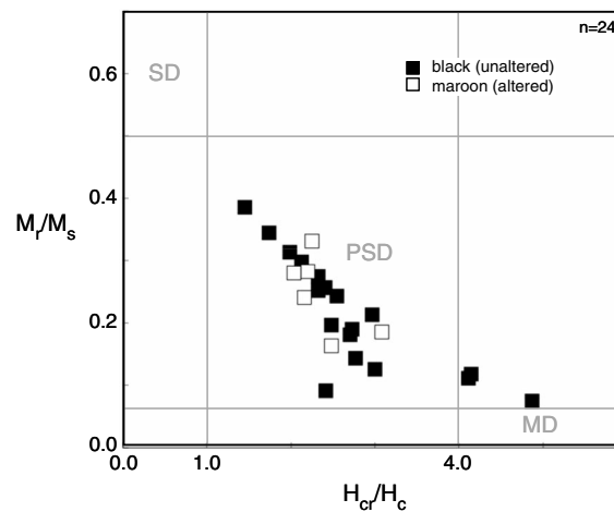
Figure 5. M_r/M_s versus H_{cr}/H_c diagram [Day et al. , 1977] for small fragments of pseudotachylytes (<3 g). Samples span along a mixing trend between SD and MD, plotting mostly in the PSD domain. The maroon, hematite-bearing specimens are statistically indistinguishable from the black, hematite-free specimens where magnetite dominates the magnetic hysteresis properties.
