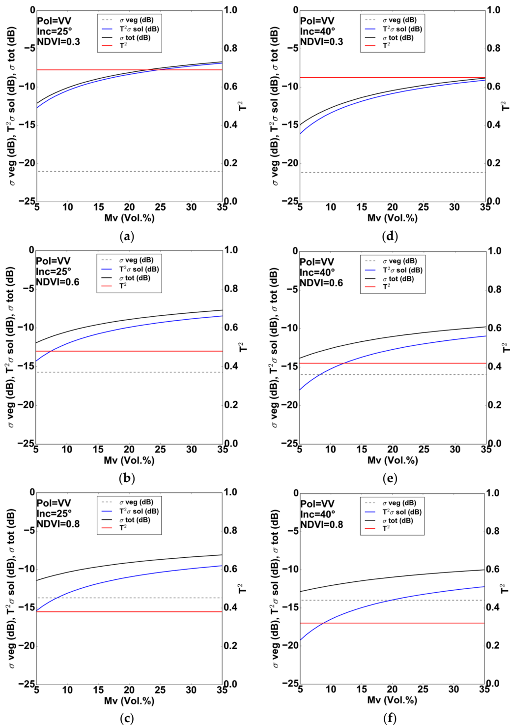
Figure 3. Behavior of WCM components ( \sigma_{veg}^0 , T^2\sigma_{soil}^0 , and \sigma_{tot}^0 ) in VV polarization according to m_v for 25° and 40° incidence angles. The soil roughness H_{rms} was fixed to 2 cm. (a): \theta = 25^\circ and NDVI = 0.3; (b): \theta = 25^\circ and NDVI = 0.6; (c): \theta = 25^\circ and NDVI = 0.8; (d): \theta = 40^\circ and NDVI = 0.3; (e): \theta = 40^\circ and NDVI = 0.6; (f): \theta = 40^\circ and NDVI = 0.8.
