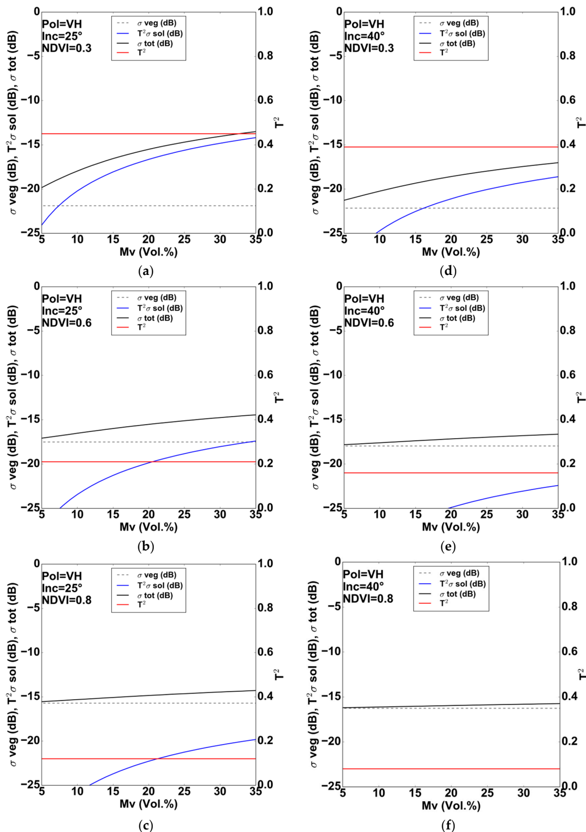
Figure 4. Behavior of WCM components ( \sigma_{veg}^0 , T^2\sigma_{soil}^0 , and \sigma_{tot}^0 ) in VH polarization according to mv for 25^\circ and 40^\circ incidence angles. The soil roughness H_{rms} was fixed to 2 cm. (a): \theta = 25^\circ and NDVI = 0.3 ; (b): \theta = 25^\circ and NDVI = 0.6 ; (c): \theta = 25^\circ and NDVI = 0.8 ; (d): \theta = 40^\circ and NDVI = 0.3 ; (e): \theta = 40^\circ and NDVI = 0.6 ; (f): \theta = 40^\circ and NDVI = 0.8 .
