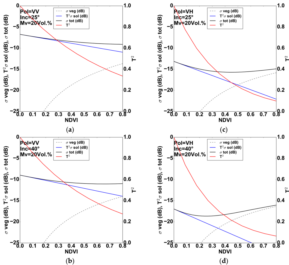
Figure 5. Behavior of WCM components ( \sigma^0_{veg} , T^2\sigma^0_{soil} , and \sigma^0_{tot} ) in VV and VH polarizations according to NDVI for 25° and 40° incidence angles, mv = 20 vol %, and Hrms = 2 cm. (a): VV and \theta = 25^\circ ; (b): VV and \theta = 40^\circ ; (c): VH and \theta = 25^\circ ; (d): VH and \theta = 40^\circ .
