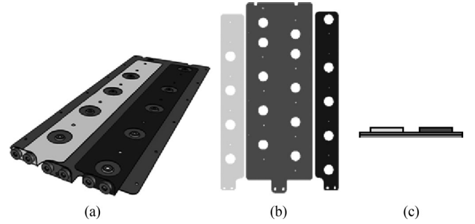
Fig. 1. (a) Three-dimensional busbar. (b) Two-dimensional conductive plates. (c) Section cut of the relative position between plates.
