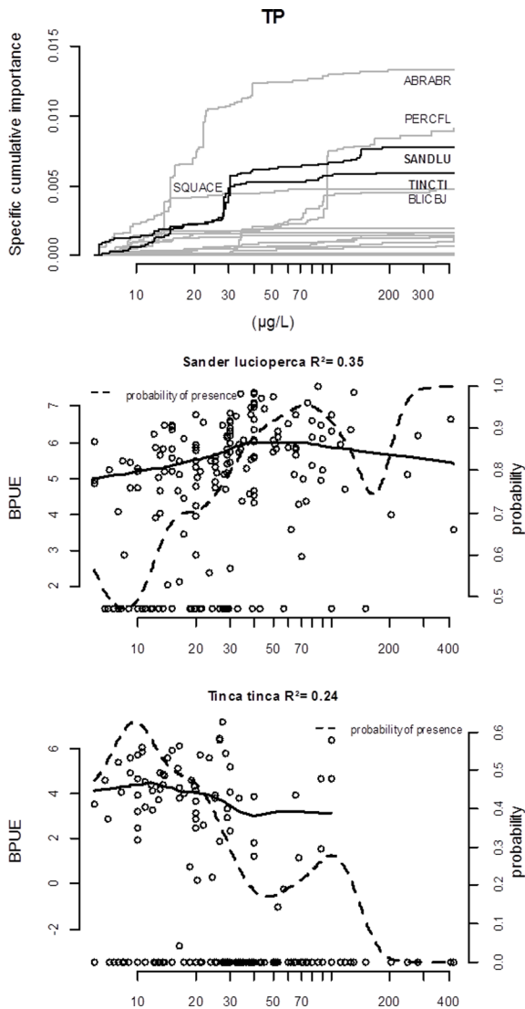
Fig. 7. Results of gradient forest for total phosphorus (TP, log scale). The specific cumulative importance indicates locations of potential thresholds in the responses of the different fish species to the gradients. Specific responses of Sander lucioperca and Tinca tinca are shown as examples. Plain lines are local regressions on strictly positive BPUE values and dashed lines are probabilities of presence along the gradients.
