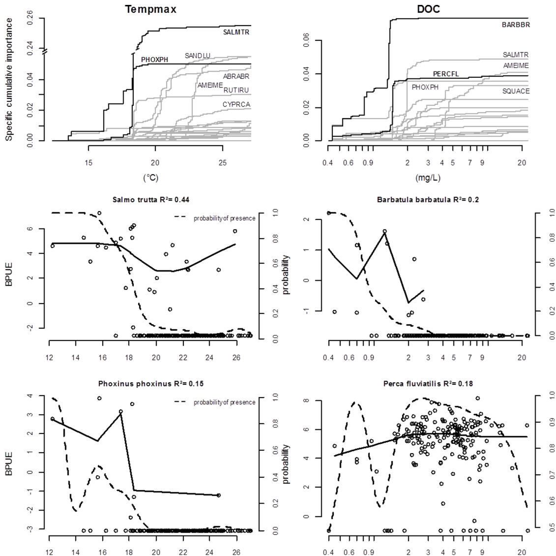
Fig. 5. Results of gradient forest for maximal water temperature (Tempmax, left column) and dissolved organic carbon (DOC, right column, log scale). The specific cumulative importance indicates the locations of potential thresholds in the responses of fish species to the gradients (note the offset of the y-axis for Salmo trutta ). The BPUE of four species are shown as examples: Salmo trutta and Phoxinus phoxinus for Tempmax and, Barbatula barbatula and Perca fluviatilis for DOC. Plain lines are local regressions on strictly positive BPUE values and dashed lines are probabilities of presence along the gradients.
