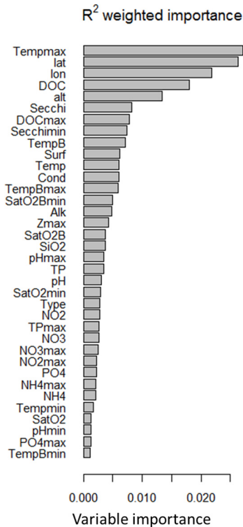
Fig. 4. Overall importance of the environmental variables for all the fish species, normalized to sum to the average specific R^2 (0.22).
