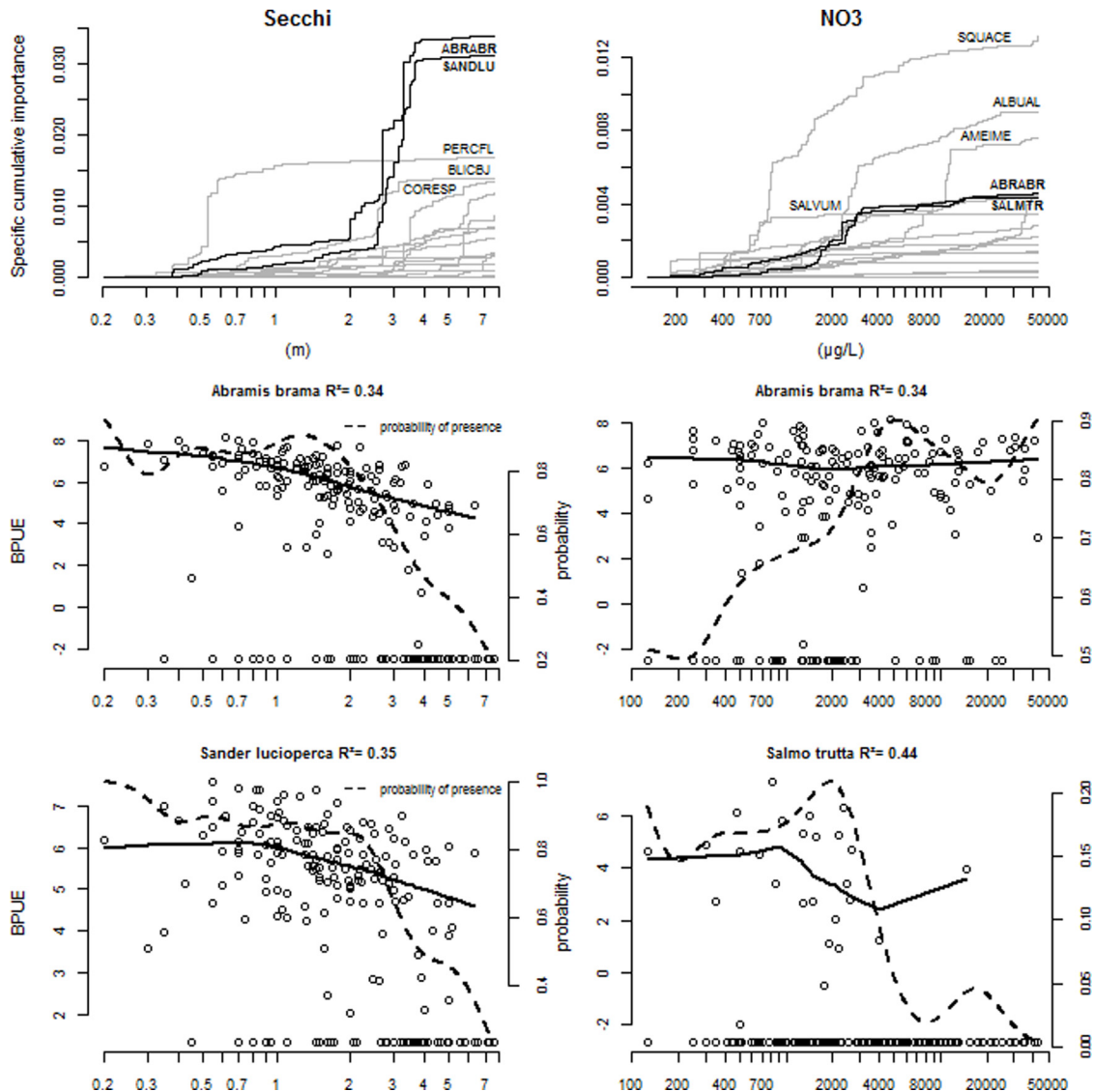
Fig. 6. Results of gradient forest for Secchi depth (Secchi, left, log scale) and median nitrate concentration (NO 3 , right, log scale). The specific cumulative importance indicates locations of potential thresholds in the responses of the different fish species to the gradients. Examples of fish responses are provided with Sander lucioperca and Salmo trutta for Secchi and NO 3 , respectively, and with Abramis brama for both variables. Plain lines are local regressions on strictly positive BPUE values and dashed lines are probabilities of presence along the gradients.
