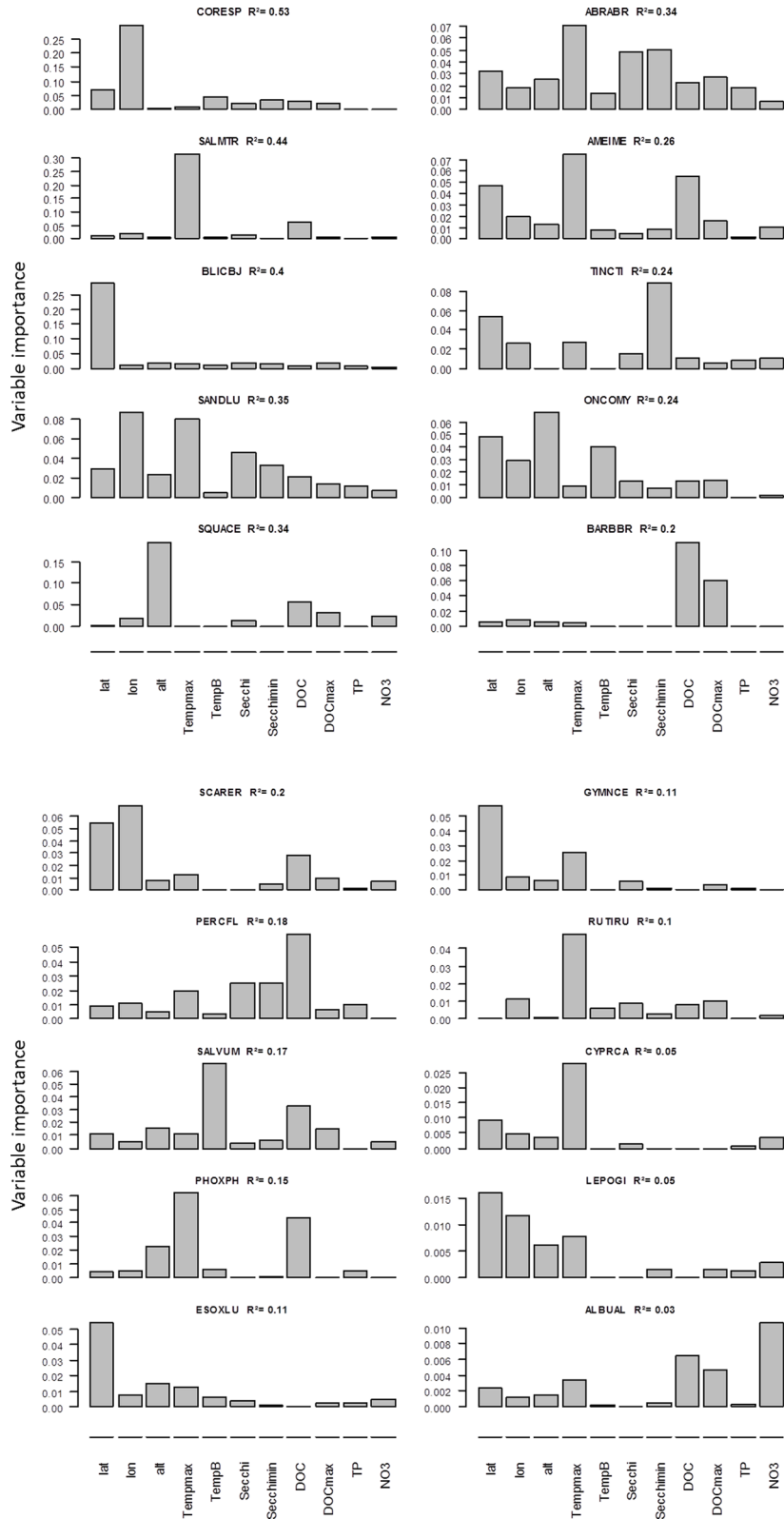
Fig. 3. Accuracy importance of the 9 most important environmental variables and the two variables NO3 and TP, for each species. Values are normalized to sum to the specific R^2 .
