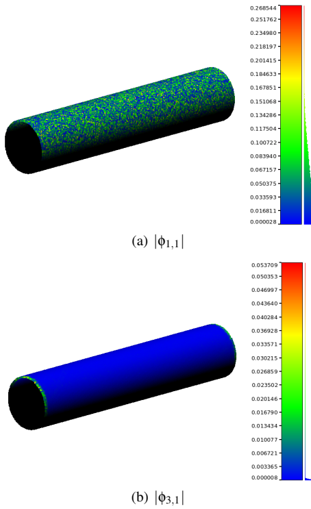
Figure 2: |\phi_{1,1}| and |\phi_{3,1}| computed on a cylinder of radius 10 with added gaussian noise on the normal direction (standard deviation of \frac{\pi}{45} .)
