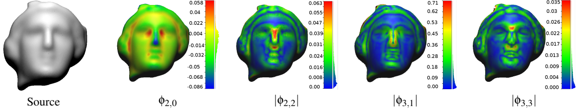
Figure 1: Computation of some values of \phi_{n,k} on a blurred face model of Caesar. |\phi_{2,2}| is globally smooth but there remains some outliers.
