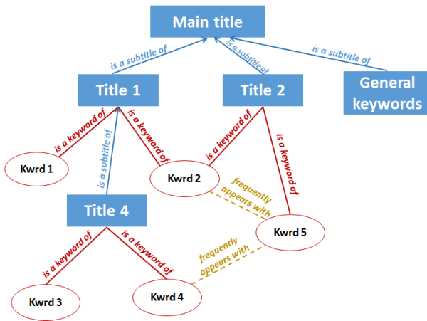
Fig. 3. Structure of the semantic graph of keywords
