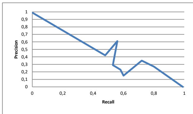
Fig. 8. Precision/Recall curve
