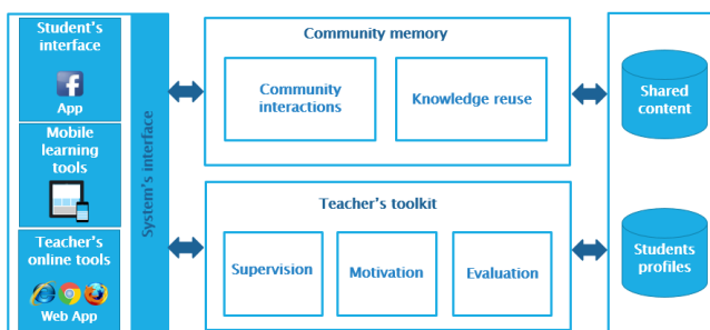
Fig. 1. General architecture of our CQA system
