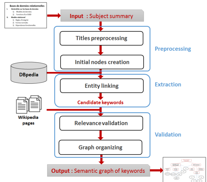
Fig. 4. The graph construction process
